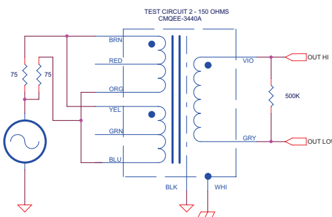
MC CARTRIDGE PHONO APPLICATIONS CMQEE-3440AHP
