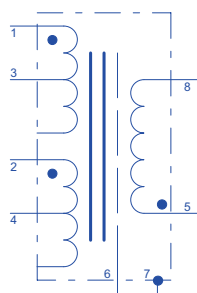
MC CARTRIDGE PHONO APPLICATIONS CMQEE-3440AHP
