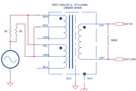
MIC/LINE APPLICATIONS CMQEE-3440APC-600
